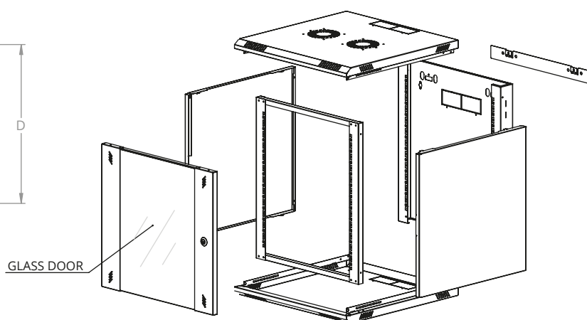
EXPLODED VIEW
