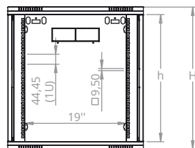
DIMENSIOIS IN WITDH AND HEIGHT
