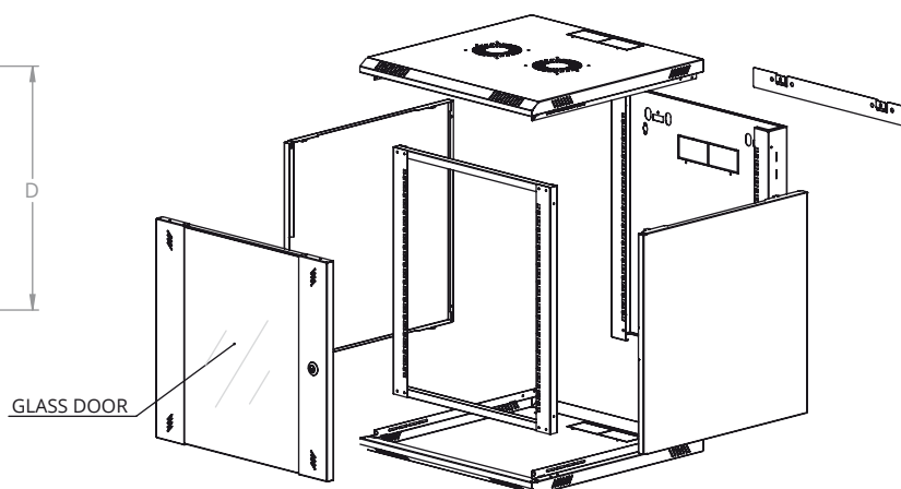
EXPLODED VIEW
