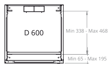
MAX/ MIN EQUIPMENT MOUNTING DISTANCE (600)
