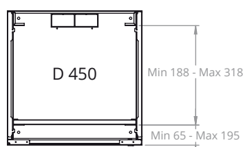
MAX/ MIN EQUIPMENT MOUNTING DISTANCE (450)
